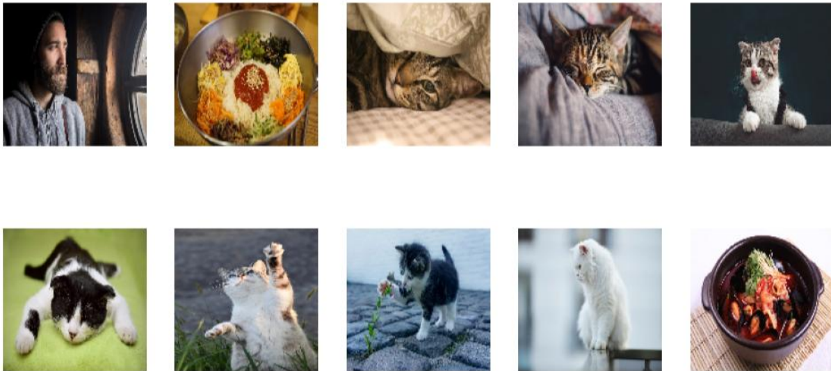
Cluster 1
